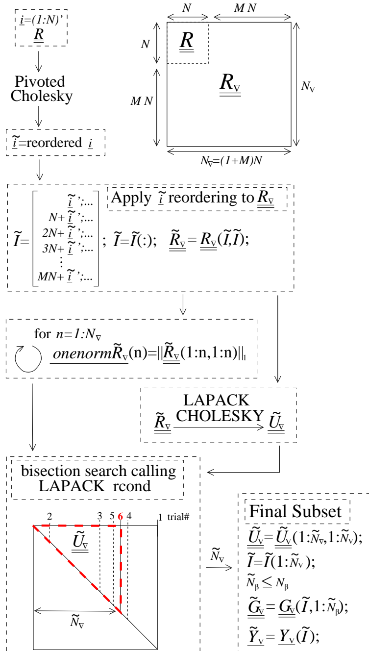
Figure 4.1: A diagram with pseudo code for the pivoted Cholesky algorithm used to select the subset of equations to retain when \underline{R}_{\nabla} is ill-conditioned. Although it is part of the algorithm, the equilibration of \underline{R}_{\nabla} is not shown in this figure. The pseudo code uses MATLAB notation.
