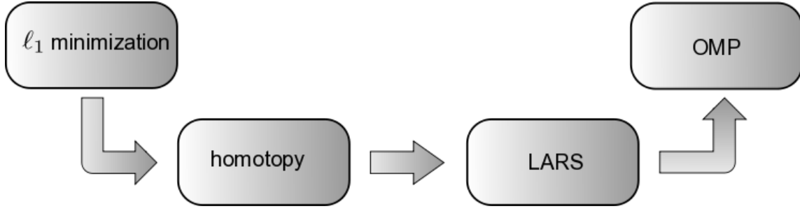
Figure 2.2: Bridging provably convergent \ell_1 minimization algorithms and greedy algorithms such as OMP. (1) Homotopy provably solves \ell_1 minimization problems [33]. (2) LARS is obtained from homotopy by removing the sign constraint check. (3) OMP and LARS are similar in structure, the only difference being that OMP solves a least-squares problem at each iteration, whereas LARS solves a linearly penalized least-squares problem. Figure and caption based upon Figure 1 in [29].
