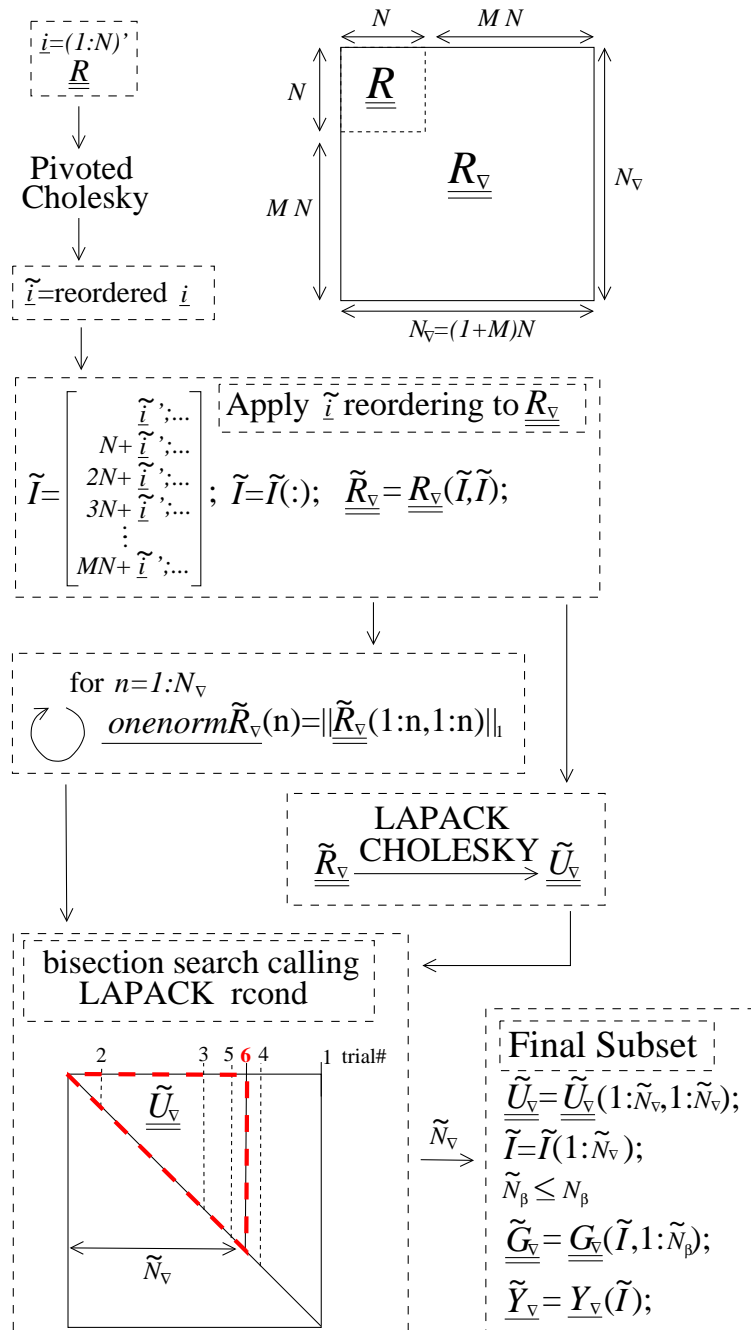
Figure 4.1: A diagram with pseudo code for the pivoted Cholesky algorithm used to select the subset of equations to retain when \underline{\underline{R}}_{\tilde{v}} is ill-conditioned. Although it is part of the algorithm, the equilibration of \underline{\underline{R}}_{\tilde{v}} is not shown in this figure. The pseudo code uses MATLAB notation.
